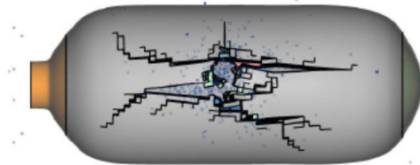
Figure 15. 300bars, 20000m/s, t=100\mu\text{s} .
