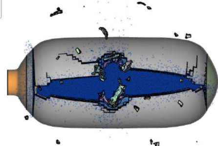
Figure 16. 300bars, 4500m/s, t=200\mu\text{s} .
