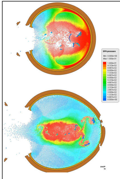
Figure 13. 2D model simulation of the tank explosion.
