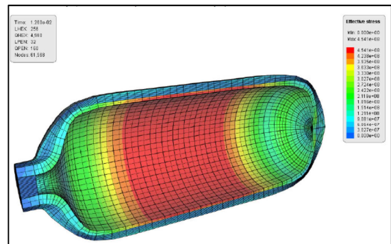
Figure 12. Tank prestress initialization.
