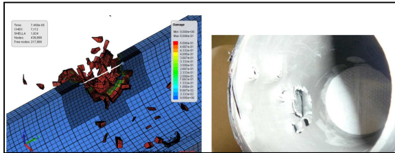
Figure 10. Simulation and experimental results.
